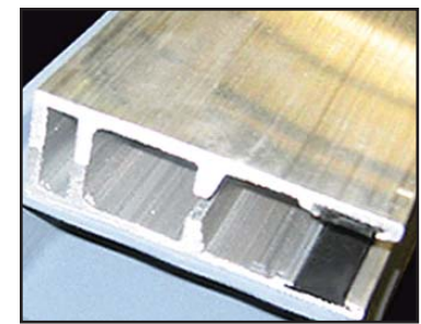
NYLON SIDE GUIDE STRIPS Eliminate metal-to-metal contact with slats.
