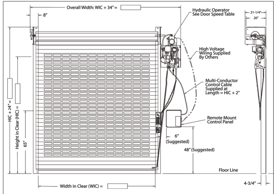
Standard dimensions shown. For tighter clearance requirements, consult factory.
